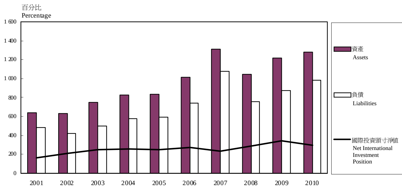
圖二 二零零一年至二零一零年的香港國際投資頭寸與以當時市價計算的本地生產總值的比率 Chart 2 Ratio of Hong Kong's International Investment Position to Gross Domestic Product (at Current Market Prices) during the period 2001 to 2010
