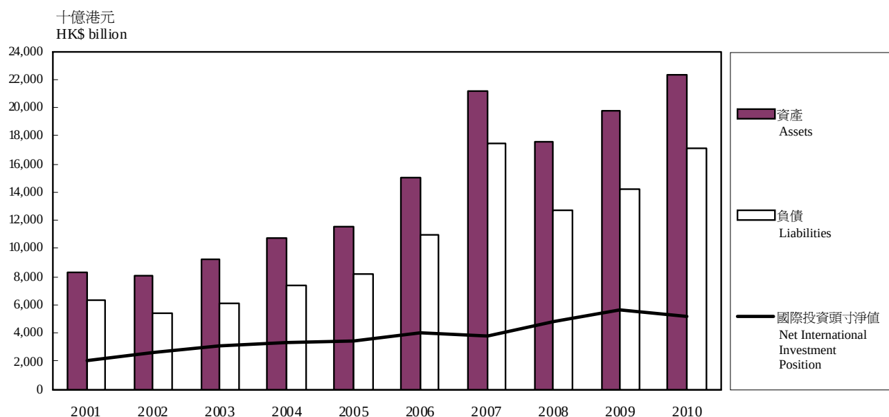
圖一 二零零一年年底至二零一零年年底的香港國際投資頭寸 Chart 1 Hong Kong's International Investment Position as at end of 2001 to 2010
